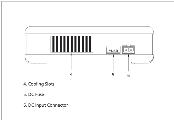
Fig. 2 - Rear view
