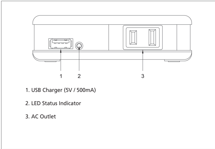
Fig. 1 - Front view
