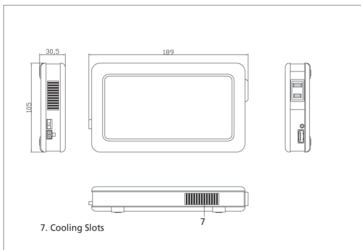
Fig. 3 - Plan, elevations & dimensions
