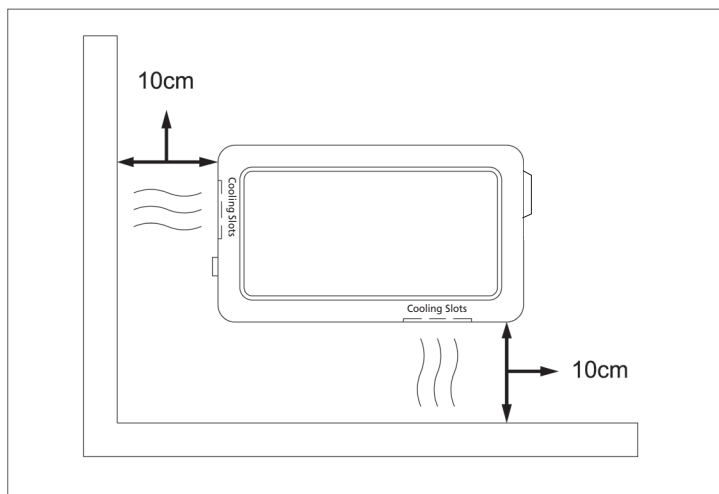
Fig. 4 - Installation clearances for installation
